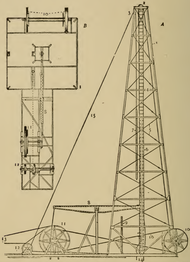
Fig. 123½. DIAGRAM OF A STEEL RIG FOR DRILLING OIL WELLS.
